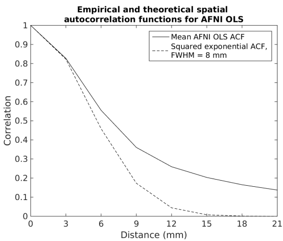
Supplementary Figure 14: Empirical versus theoretical spatial autocorrelation functions (SACFs) for a) SPM, b) FSL and c) AFNI. The SACFs were estimated and averaged using 1,000 group difference maps, generated from two sample t -tests (10 subjects per group) using the Beijing data (analyzed with the E2 paradigm and 6 mm smoothing). Note that the empirical SACFs have a much longer tail compared to the theoretical squared exponential SACF, thereby violating one of the required assumptions for parametric cluster-wise inference using Gaussian random field theory. Both SPM and FSL resample the fMRI data to a resolution of 2 mm, while AFNI instead uses a resolution of 3 mm for the specific datasets. For this reason, the SACFs are sampled differently for AFNI.
